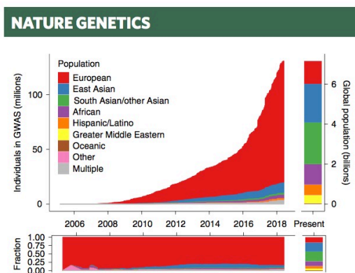
Fig. 1 | Ancestry of GWAS participants over time, as compared with the global population. Cumulative data, as reported by the GWAS catalog 76 . Individuals whose ancestry is 'not reported' are not shown.
